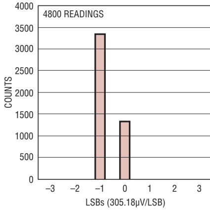
Single-Ended Noise
